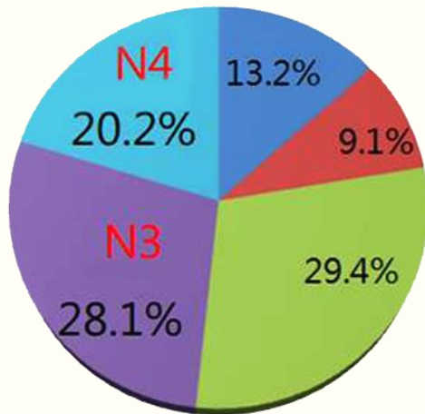
N3以上達48.3% (431/892)
